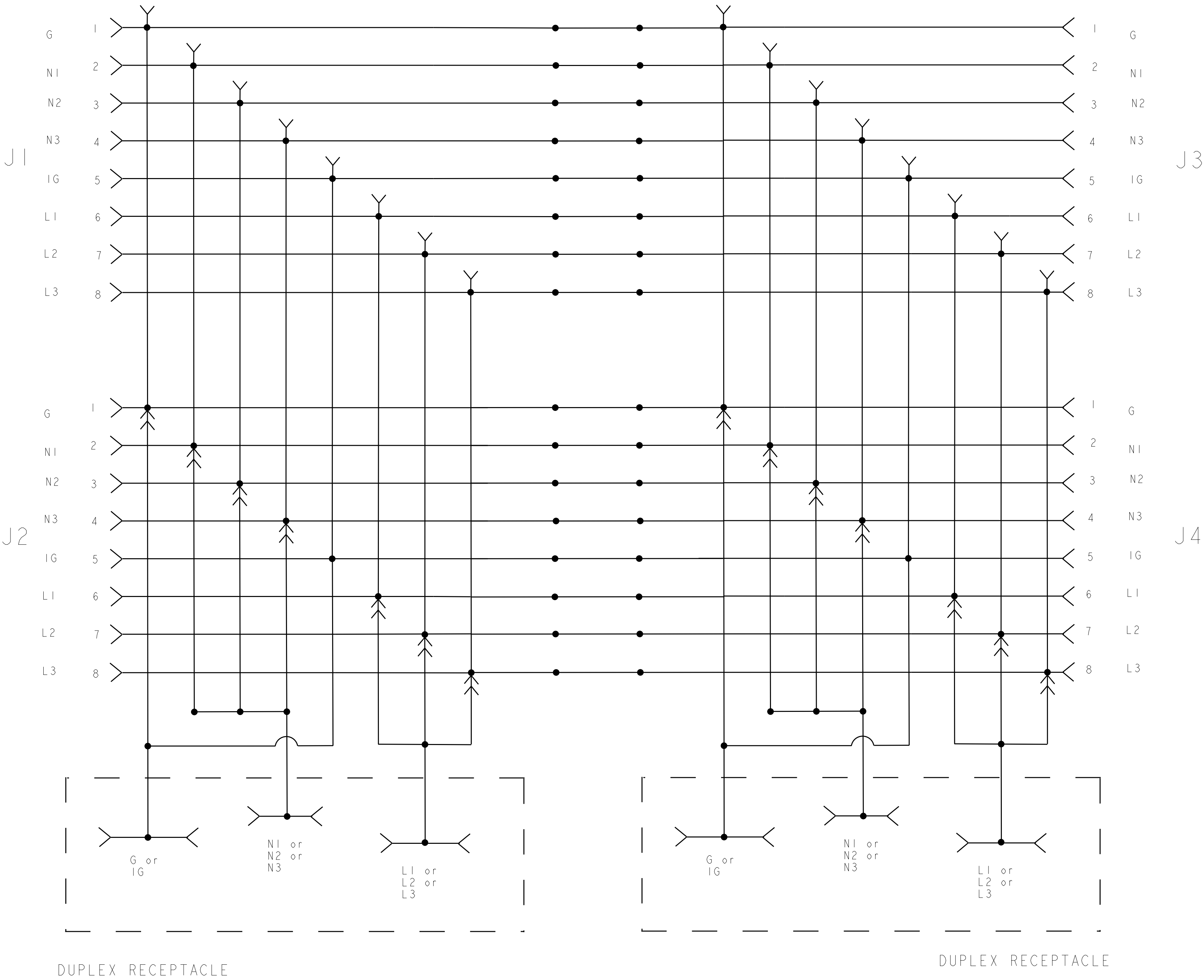
ELECTRICAL SCHEMATIC FOR 8-WIRE, DEDICATED NEUTRAL (3-3-2) POWER STRIP ⚠
