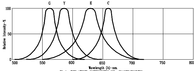
Fig1. RELATIVE INTENSITY VS. WAVELENGTH
