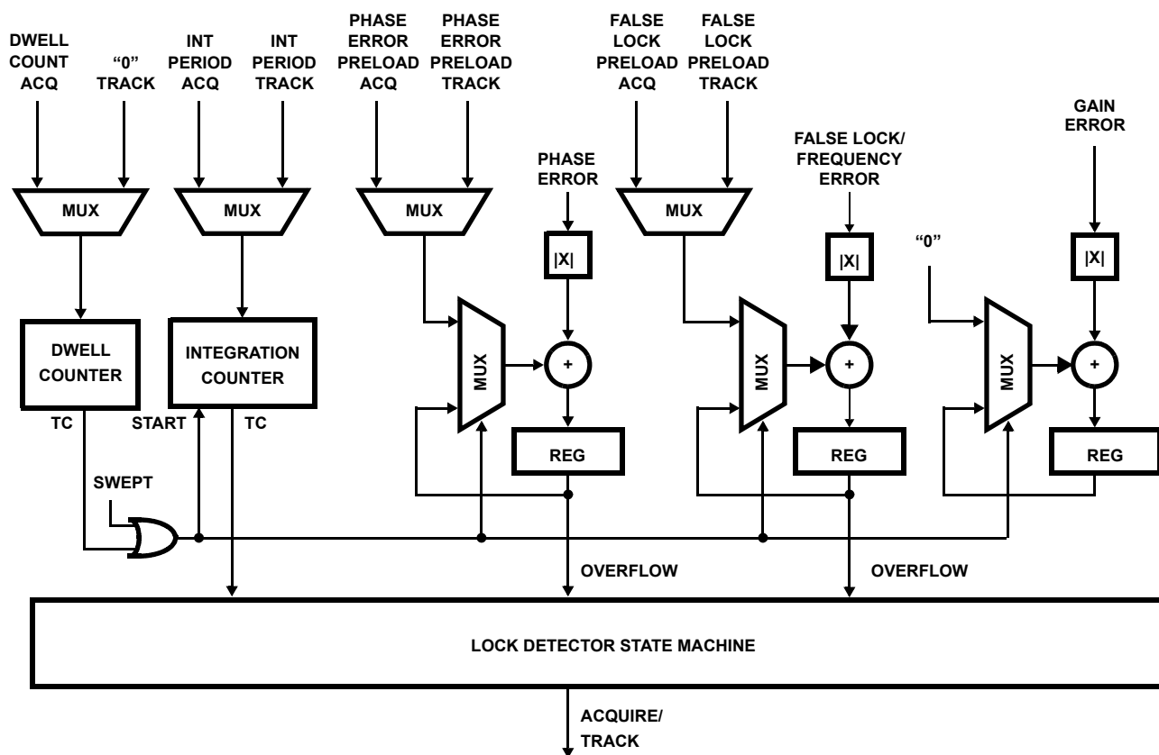
FIGURE 17. LOCK DETECTOR BLOCK DIAGRAM
