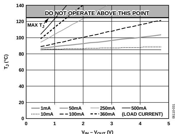
Figure 43. 300 mm² of PCB Copper, T_A = 85^\circ C
