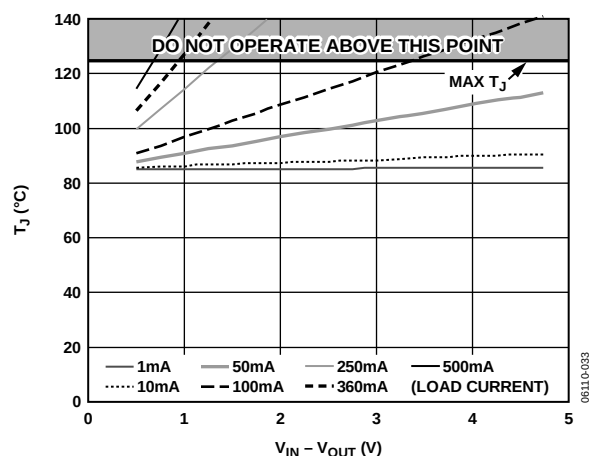
Figure 45. 0 mm² of PCB Copper, T_A = 85^\circ C
