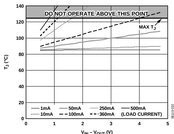
Figure 44. 100 mm² of PCB Copper, T_A = 85^\circ C
