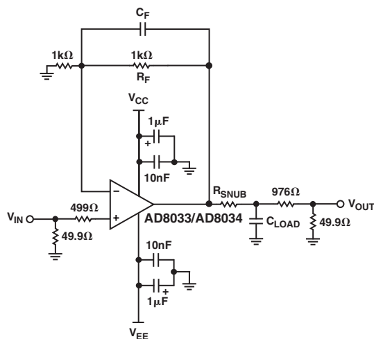
Test Circuit 2. G = +2
