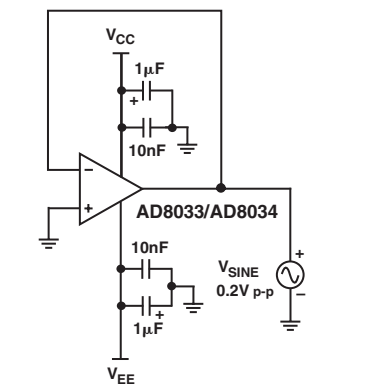
Test Circuit 4. Output Impedance G = +1
