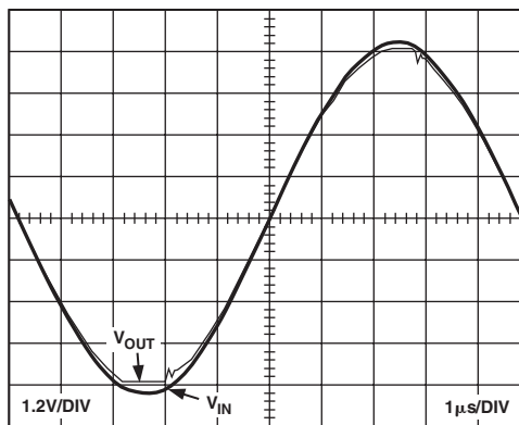
TPC 38. G = +2 Response V_S = \pm 5\text{ V}
