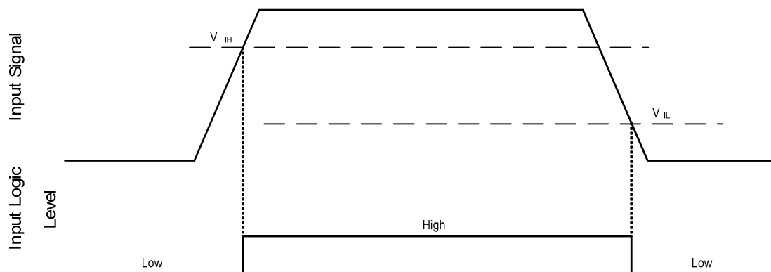
Figure 7: HIN & LIN input thresholds
