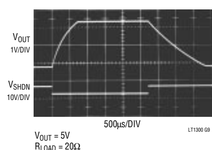
Startup Response
