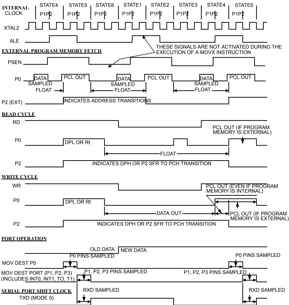
Figure 26. Clock Waveforms
