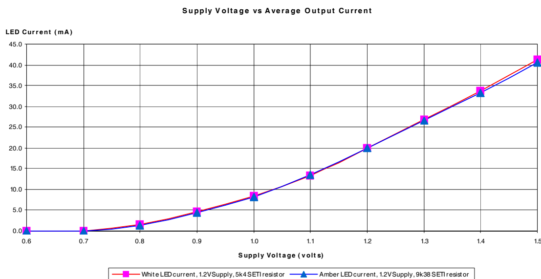
Fig.14 Variation of output current against supply voltage.
