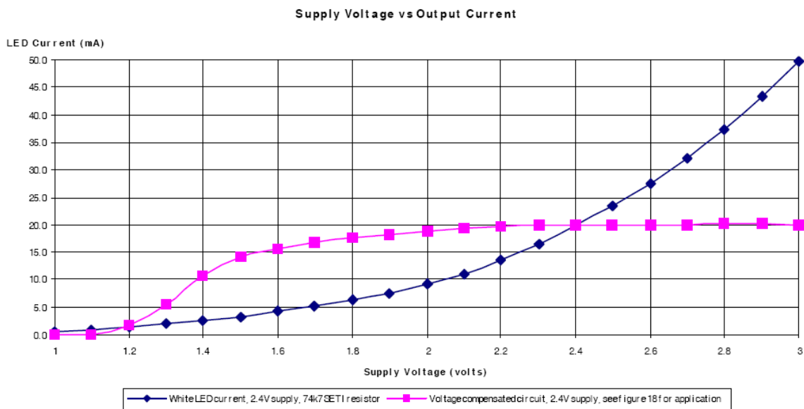
Fig.16 LED current against supply voltage, showing stabilized and uncompensated curves (fig 15 & 4).
