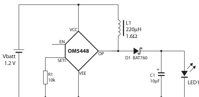
Fig.4 DC driven LED circuit
