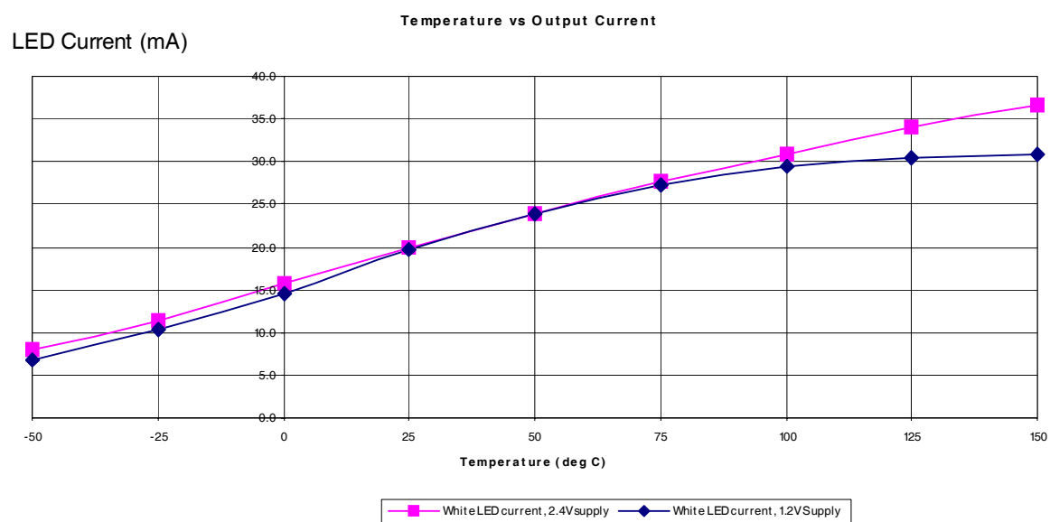
Fig.17 LED current against temperature. White LED, circuit figure 4.
