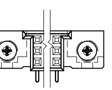
SPECIAL FEATURE OPTION "D" SEE NOTE 6
