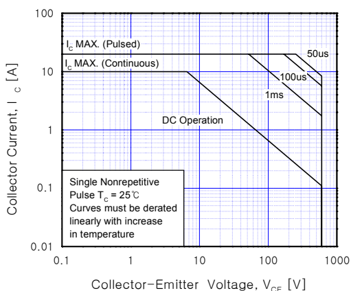
Figure 15. SOA Characteristics
