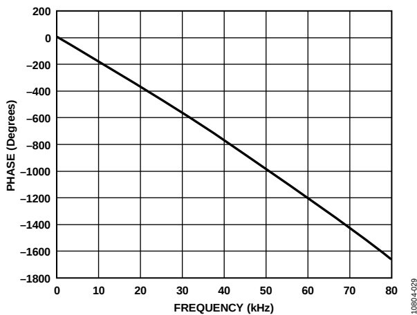
Figure 30. Phase vs. Frequency, 80 kHz Bandwidth, f_s = 192 kHz, Signal Path = AIN0 to ASRC to ADC_SDAT00
