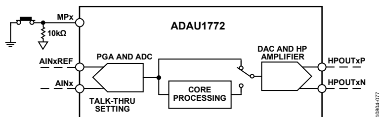
Figure 93. DSP Bypass Path Enabled
