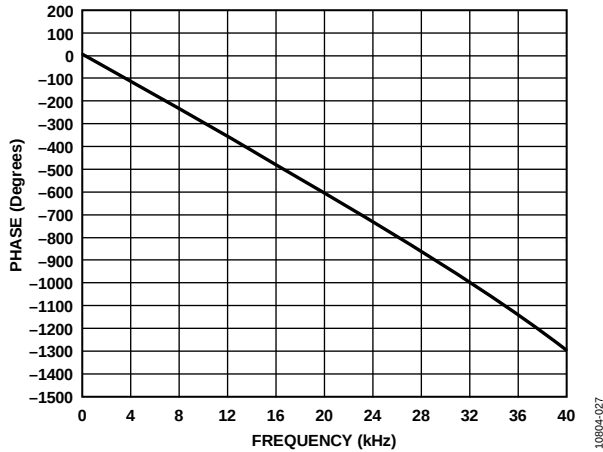
Figure 28. Phase vs. Frequency, 40 kHz Bandwidth, f_s = 96 kHz, Signal Path = AIN0 to ASRC to ADC_SDAT00
