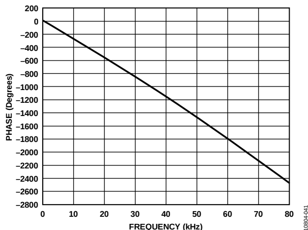
Figure 42. Phase vs. Frequency, 80 kHz Bandwidth, f_s = 192 kHz, Signal Path = DAC_SDATA to ASRC to LOU TLx
