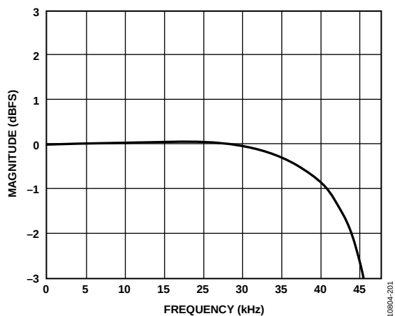
Figure 64. Decimation Pass-Band Response, Core f_s = 96 kHz, Serial Port f_s = 96 kHz
