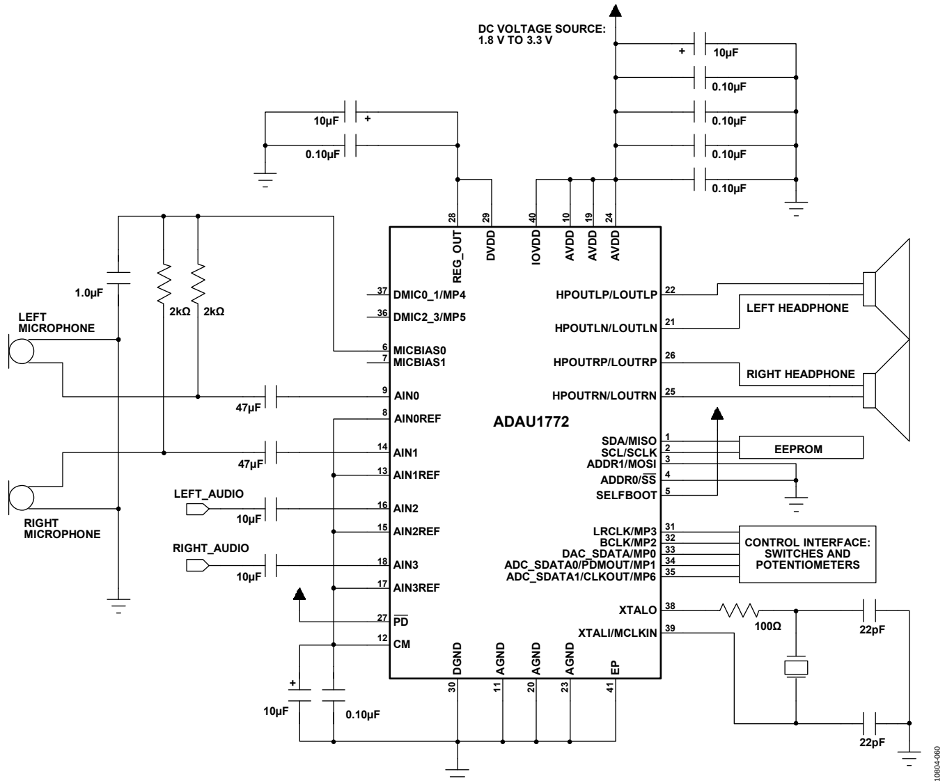
Figure 75. ADAU1772 System Block Diagram with Analog Microphones, Self-Boot Mode
