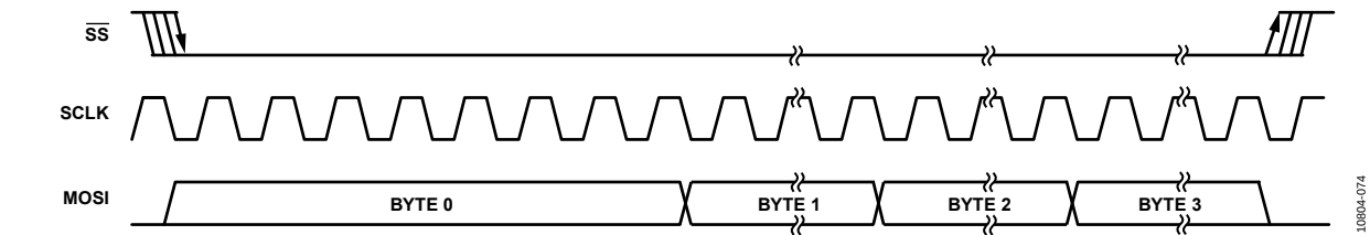
Figure 89. SPI Write to ADAU1772 Clocking (Single-Write Mode)
