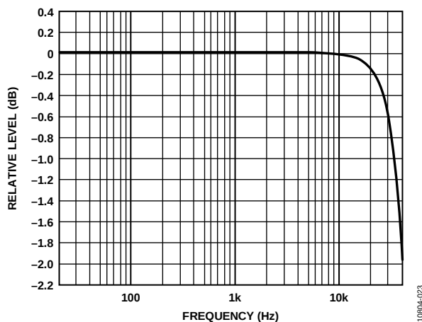
Figure 24. Relative Level vs. Frequency, f_s = 96 kHz, Signal Path = AIN0 to ASRC to ADC_SDATA0
