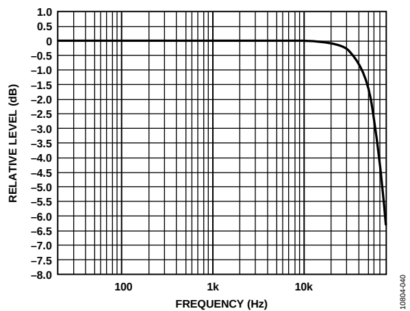
Figure 41. Relative Level vs. Frequency, f_s = 192 kHz, Signal Path = DAC_SDATA to ASRC to LOU TLx
