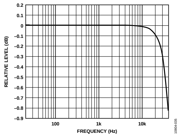
Figure 36. Relative Level vs. Frequency, f_s = 96 kHz, Signal Path = DAC_SDATA to ASRC to LOU TLx
