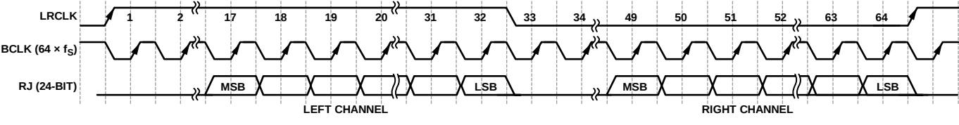
Figure 97. Right Justified Mode—16 Bits per Channel
