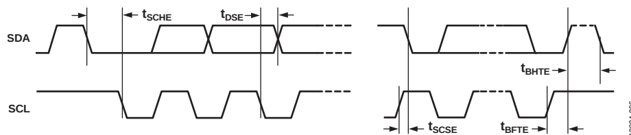
Figure 6. I²C Self-Boot Timing
