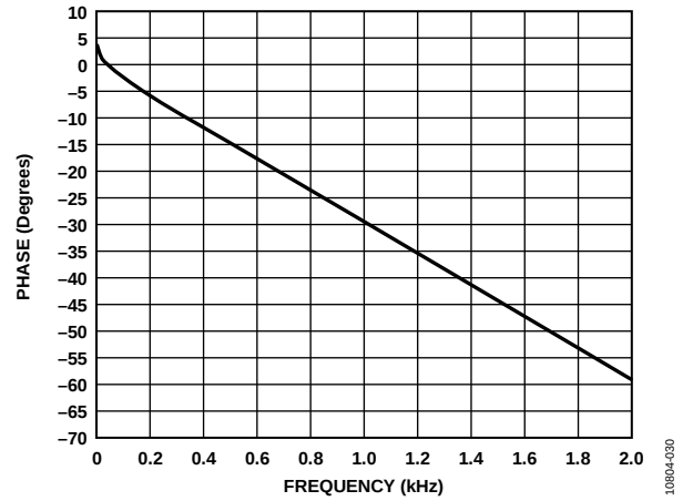
Figure 31. Phase vs. Frequency, 2 kHz Bandwidth, f_s = 96 kHz, Signal Path = AIN0 to ASRC to ADC_SDAT00
