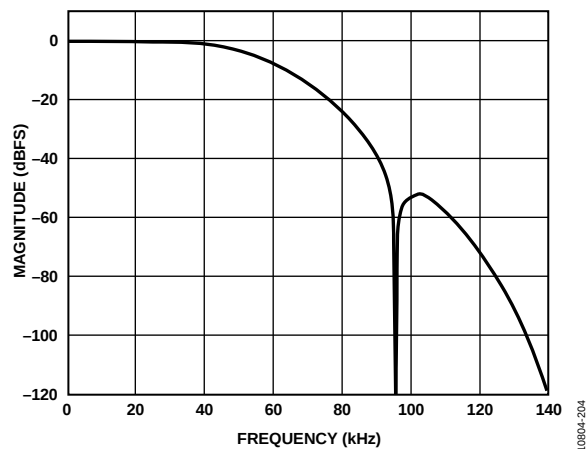
Figure 67. Total Decimation Response, Core f_s = 96 kHz, Serial Port f_s = 192 kHz
