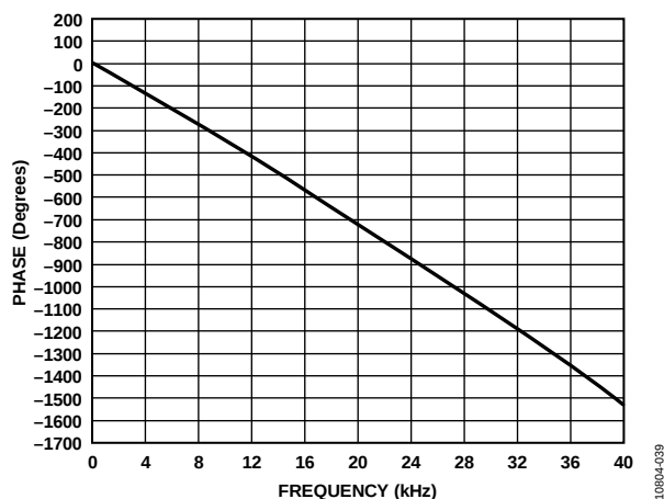
Figure 40. Phase vs. Frequency, 40 kHz Bandwidth, f_s = 96 kHz, Signal Path = DAC_SDATA to ASRC to LOU TLx
