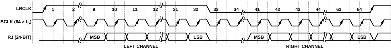
Figure 96. Right Justified Mode—24 Bits per Channel
