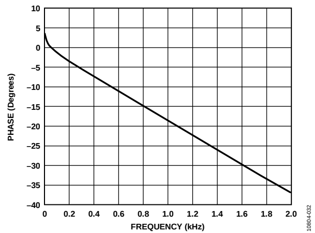
Figure 33. Phase vs. Frequency, 2 kHz Bandwidth, f_s = 192 kHz, Signal Path = AIN0 to ASRC to ADC_SDAT00
