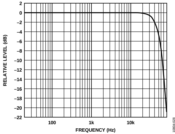
Figure 29. Relative Level vs. Frequency, f_s = 192 kHz, Signal Path = AIN0 to ASRC to ADC_SDAT00
