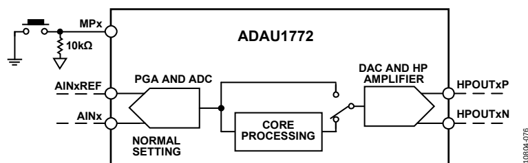
Figure 92. DSP Bypass Path Disabled
