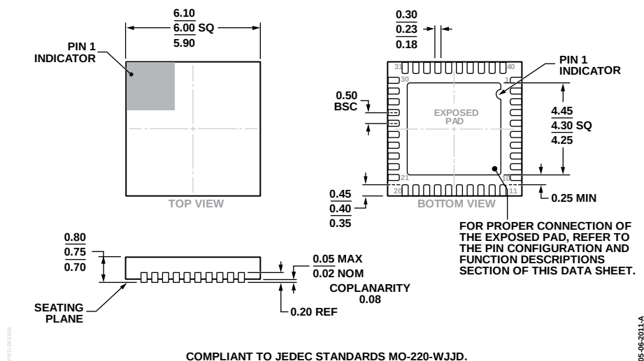
Figure 105. 40-Lead Lead Frame Chip Scale Package [LFCSP_WQ] 6 mm × 6 mm Body, Very Very Thin Quad (CP-40-10) Dimension shown in millimeters
