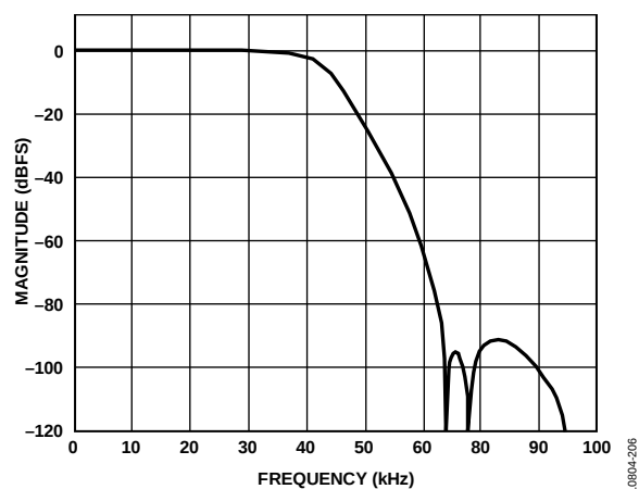
Figure 69. Total Decimation Response, Core f_s = 192 kHz, Serial Port f_s = 96 kHz
