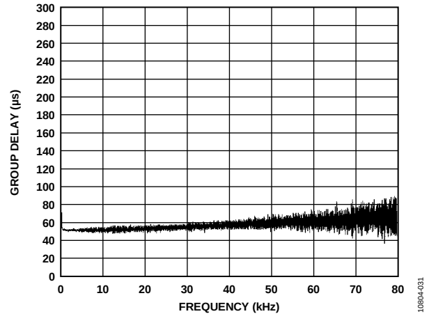
Figure 32. Group Delay vs. Frequency, f_s = 192 kHz, Signal Path = AIN0 to ASRC to ADC_SDAT00
