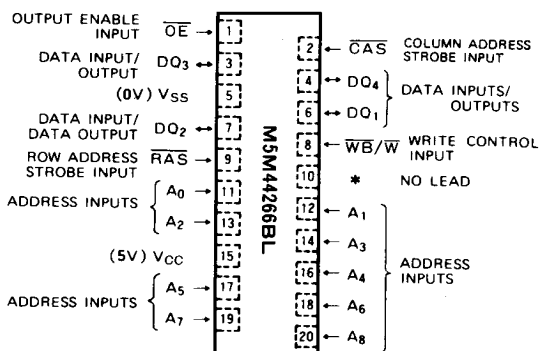
Outline 20P5L-A(ZIP)
