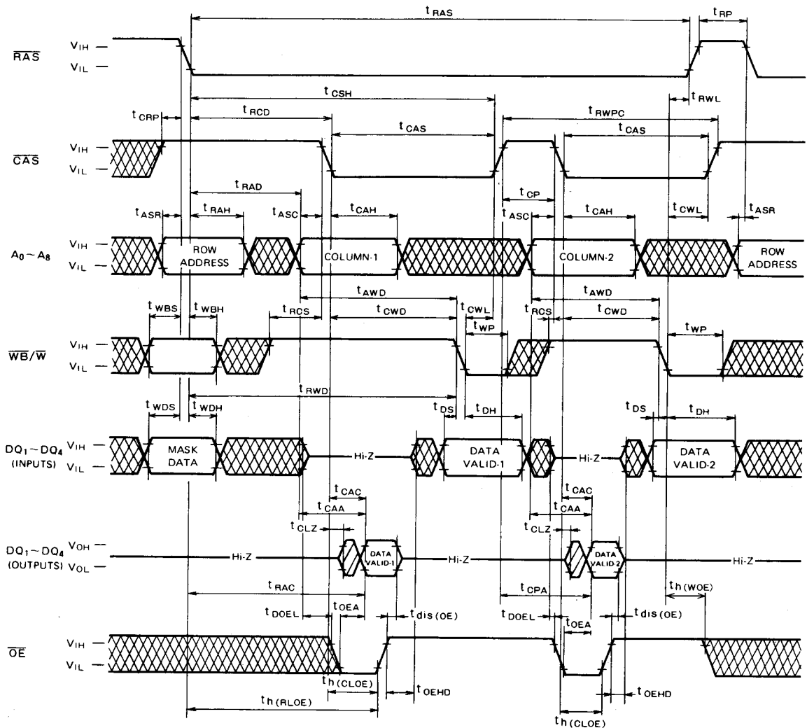
Fast Page Mode Read-Write, Read-Modify-Write Cycle (Note 27)
