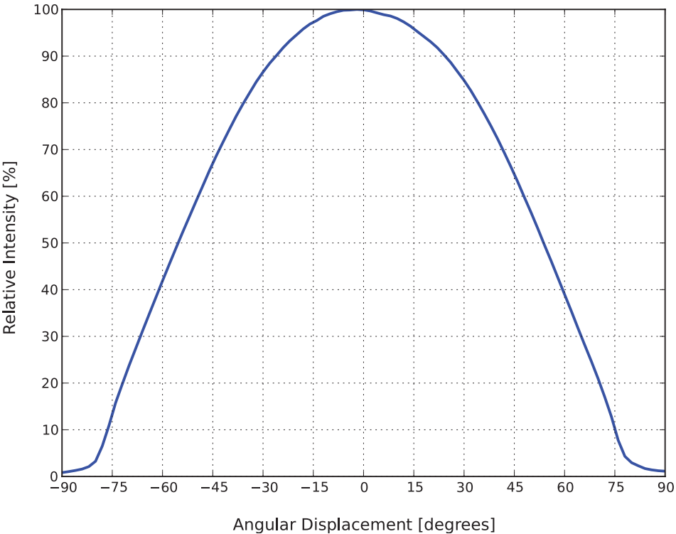
Figure 6. Typical representative spatial radiation pattern for LX5x-PWxx.
