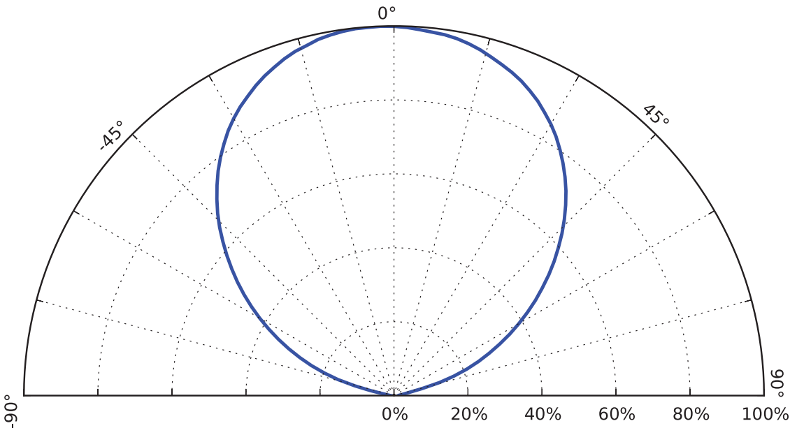
Figure 7. Typical representative polar radiation pattern for LX5x-PWxx.
