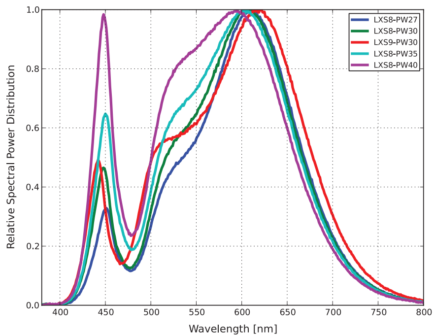
Figure 2. Color Spectra of LXSx-PWxx.
