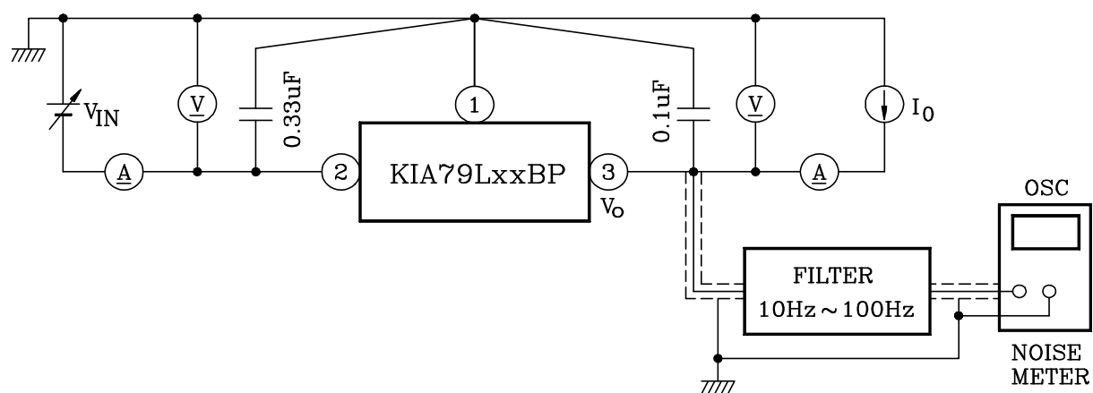
TEST CIRCUIT 3
