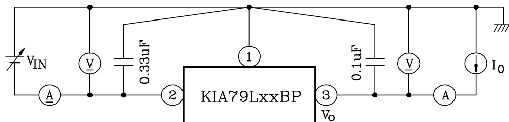
TEST CIRCUIT 1
