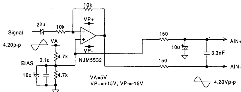
Figure 7. Single-ended Input Buffer Circuit Example
