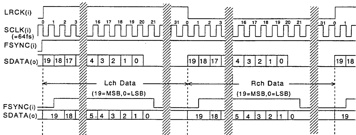
Figure 1. Data Output Timing (Slave mode)
