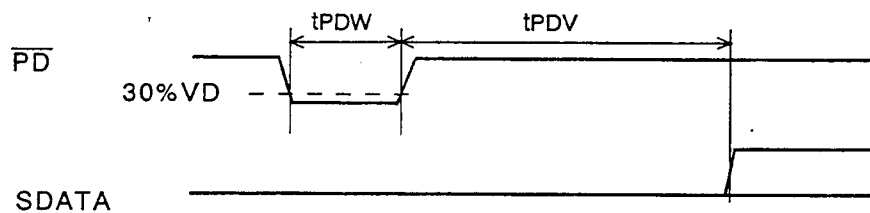
POWER DOWN TIMING
