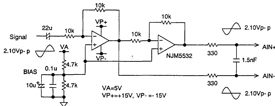
Figure 6. Full-differential Input Buffer Circuit Example
