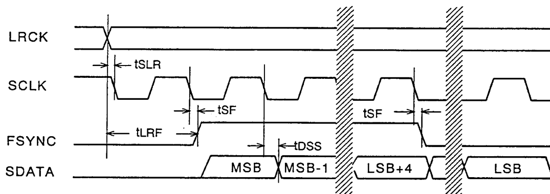
SERIAL DATA TIMING (MASTER MODE)
