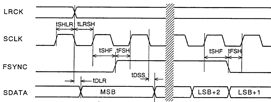
SERIAL DATA TIMING (SLAVE MODE)
