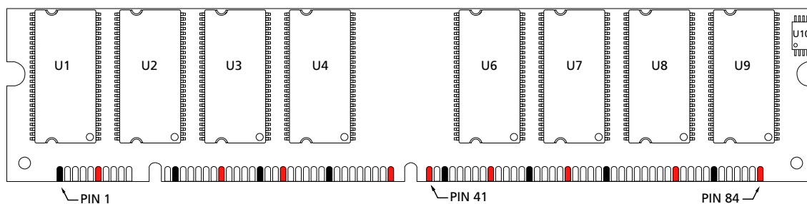
Figure 2: 168-Pin DIMM Pin Locations
