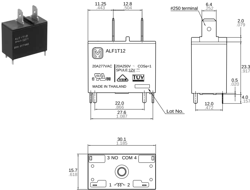
External dimensions
