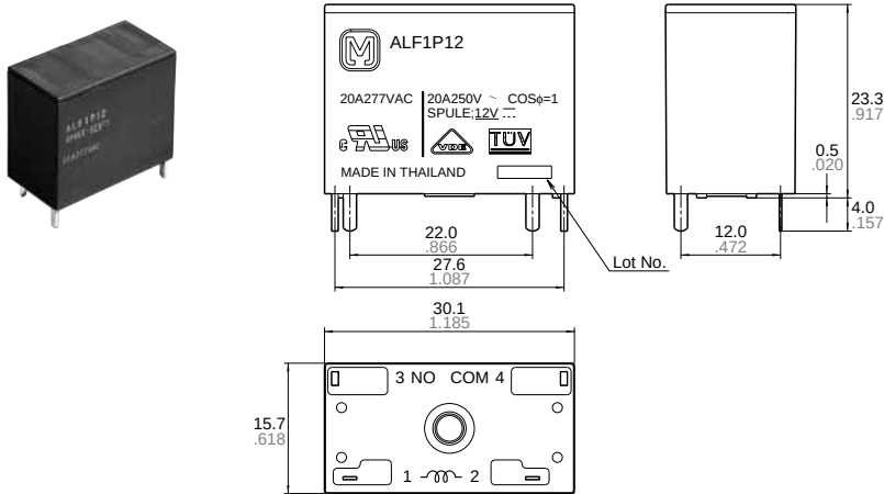
External dimensions
