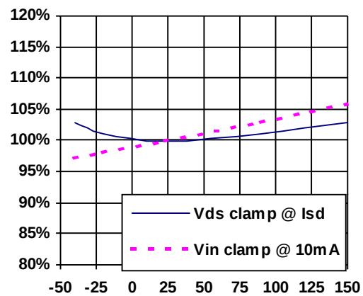
Figure 18 - Vin clamp and V clamp2 (V) Vs Tjunction ( ^{\circ} C)
