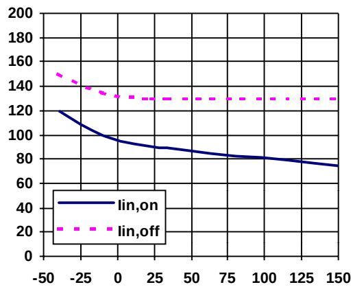
Figure 17 - Input current ( \mu A) Vs Junction ( ^{\circ} C)
