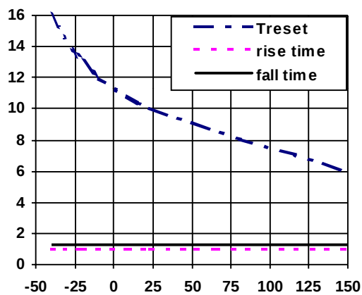
Figure 19 - Turn-on, Turn-off, and Treset ( \mu s) Vs Tjunction ( ^{\circ} C)
