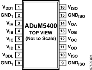
Figure 3. Pin Configuration
