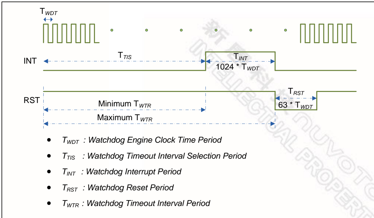
Figure 5-10 Timing of Interrupt and Reset Signals
