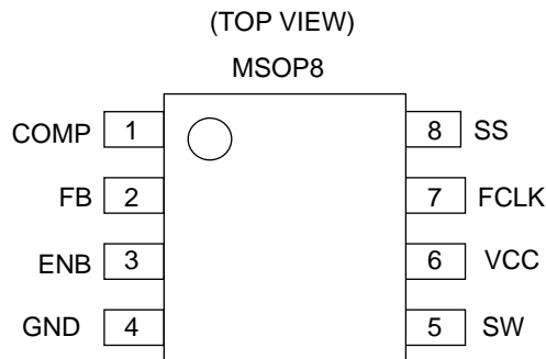
Figure 2. Pin Configuration
