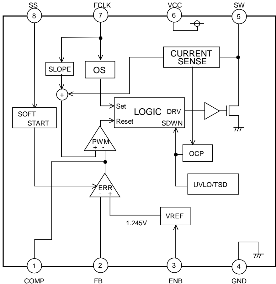
Figure 3. Block Diagram
