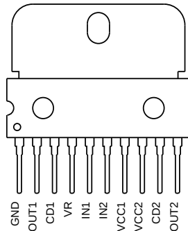
Fig.16 HSIP10
