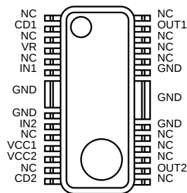
Fig.14 HSOP25
