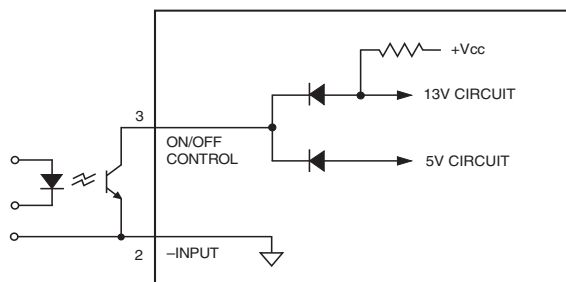
Figure 2. Internal On/Off Control circuitry
