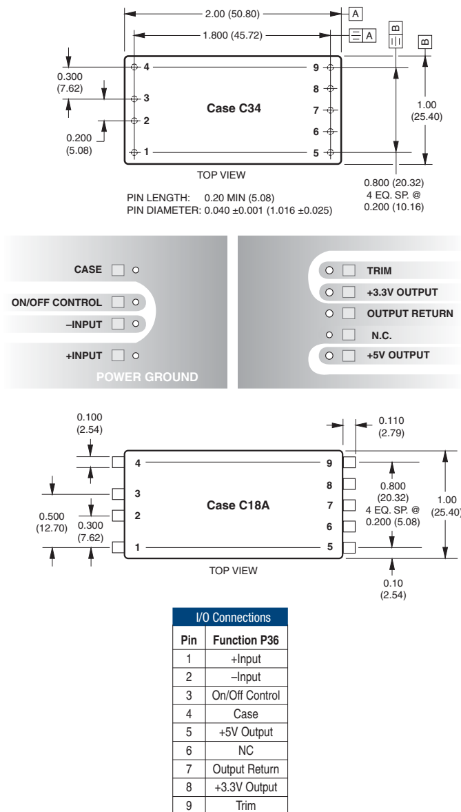
Figure 6. Recommended Board Layout
