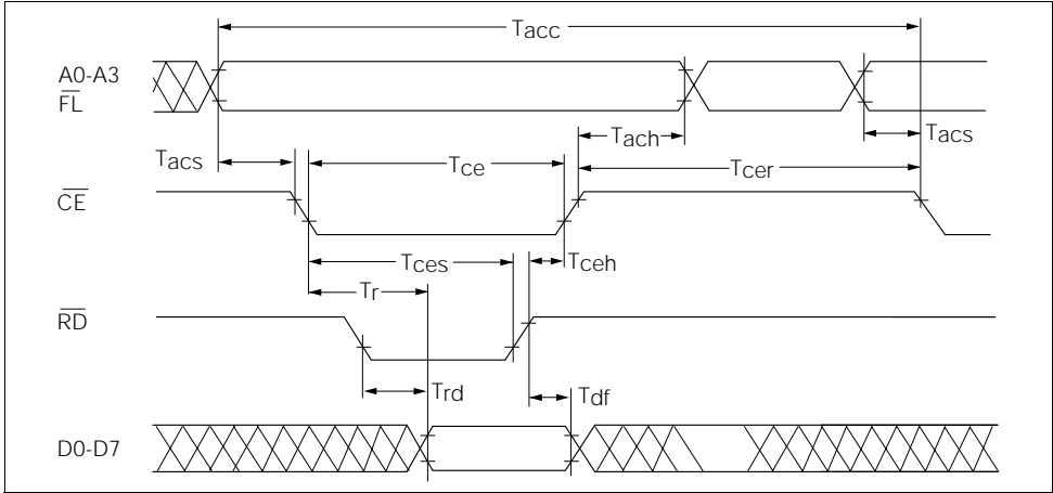
Read Cycle Timing Diagram
