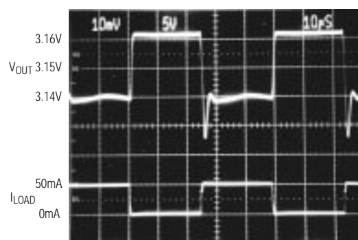
LOAD-TRANSIENT RESPONSE
