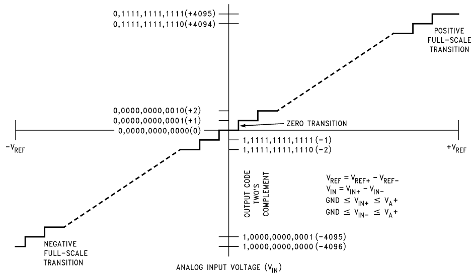
Figure 9. Transfer Characteristic
