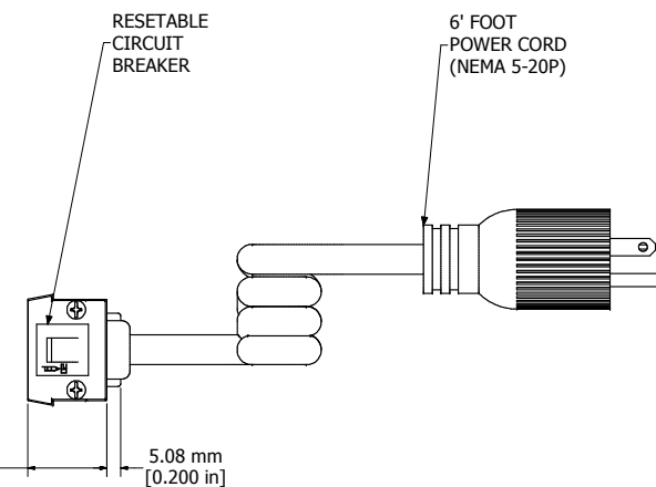
ASSEMBLY - VIEW FROM END
