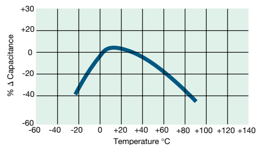
Temperature Coefficient
