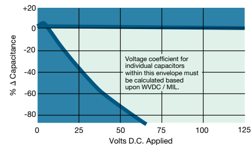
Voltage Coefficient
