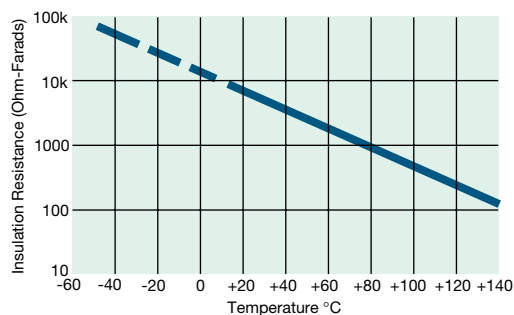
Insulation Resistance vs. Temp.
