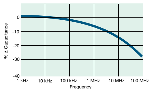
\Delta Capacitance vs. Frequency
