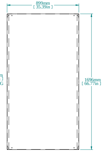
INNER PANEL
