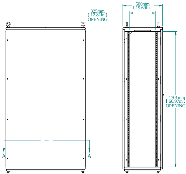
L.S. VIEW
