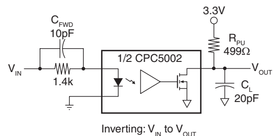
Figure 1. Inverting Configuration
