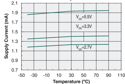
Typical Supply Current vs. Temperature
