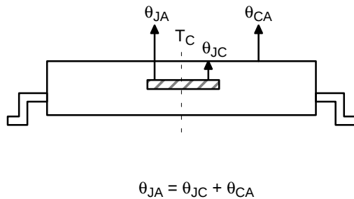
Figure 13. Thermal Resistance — °C/Watt
