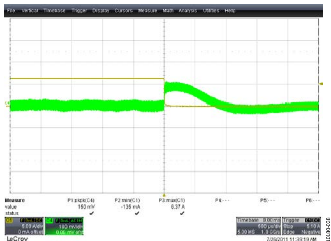
Figure 39. Output Voltage Transient, 25% to 0% Load, 385 V DC, One Phase Only Yellow Trace: Load Current, 5 A/div, 500 µs/div Green Trace: Output Voltage (AC-Coupled), 100 mV/div, 500 µs/div
