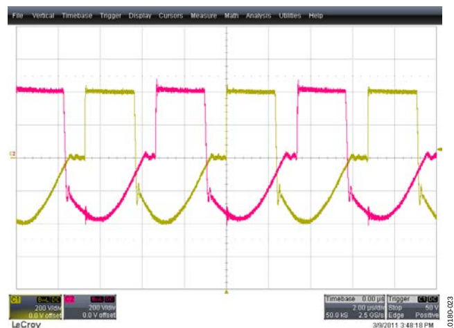
Figure 24. Transformer Primary Waveform at 25 A Load, 400 V DC Red Trace: Voltage Across T1 Primary (Phase 1), 200 V/div, 2 µs/div Yellow Trace: Voltage Across T2 (Phase 2), 200 V/div, 2 µs/div
