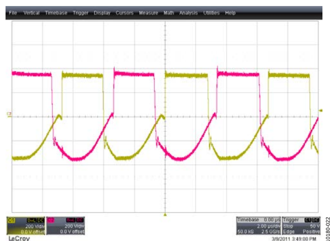
Figure 23. Transformer Primary Waveform at 25 A Load, 350 V DC Red Trace: Voltage Across T1 Primary (Phase 1), 200 V/div, 2 µs/div Yellow Trace: Voltage Across T2 (Phase 2), 200 V/div, 2 µs/div
