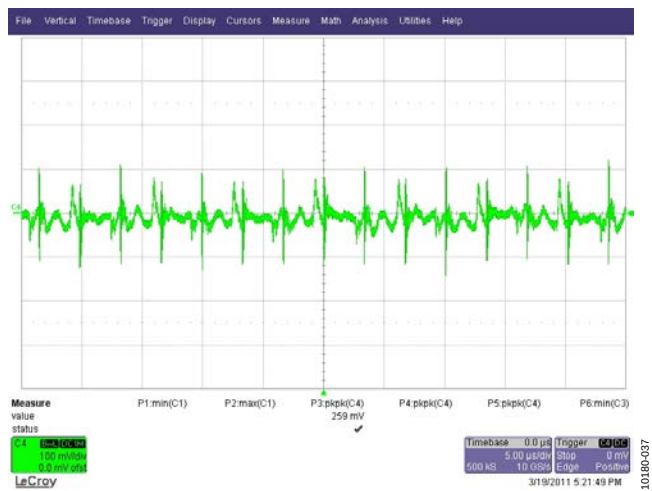
Figure 38. Output Voltage at 2700 µF Capacitor C10 (AC-Coupled), 385 V DC, 25 A, 100 mV/div, 5 µs/div, High Frequency Component
