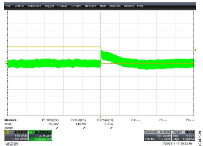
Figure 40. Output Voltage Transient, 25% to 0% Load, 385 V DC, Both Phases Active Yellow Trace: Load Current, 5 A/div, 500 µs/div Green Trace: Output Voltage (AC-Coupled), 100 mV/div, 500 µs/div
