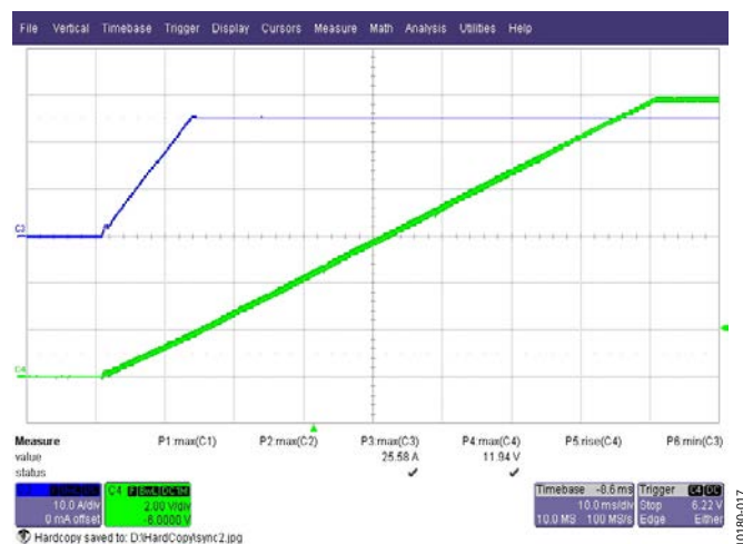
Figure 18. Startup at 385 V DC, 25 A Load (1 A/μs Slew Rate) Green Trace: Output Voltage, 2 V/div, 10 ms/div Blue Trace: Load Current, 10 A/div, 10 ms/div
