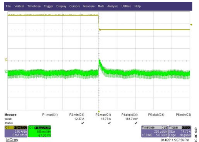
Figure 50. Output Voltage Transient, 75% to 50% Load, 385 V DC, Both Phases Active Yellow Trace: Load Current, 5 A/div, 200 μs/div Green Trace: Output Voltage (AC-Coupled), 100 mV/div, 200 μs/div
