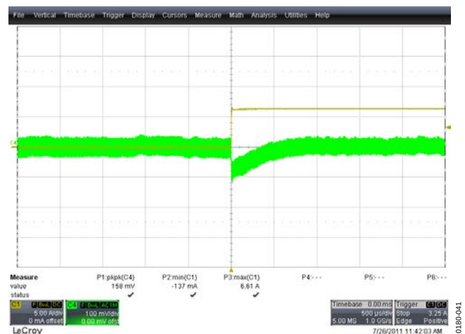
Figure 42. Output Voltage Transient, 0% to 25% Load, 385 V DC, Both Phases Active Yellow Trace: Load Current, 5 A/div, 500 µs/div Green Trace: Output Voltage (AC-Coupled), 100 mV/div, 500 µs/div
