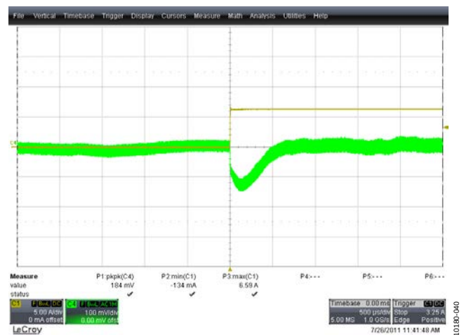
Figure 41. Output Voltage Transient, 0% to 25% Load, 385 V DC, One Phase Only Yellow Trace: Load Current, 5 A/div, 500 µs/div Green Trace: Output Voltage (AC-Coupled), 100 mV/div, 500 µs/div
