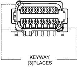
P/N ATF13-12PD-BM0X KEY-D CONFIGURATION STANDARD COLOR: BROWN
