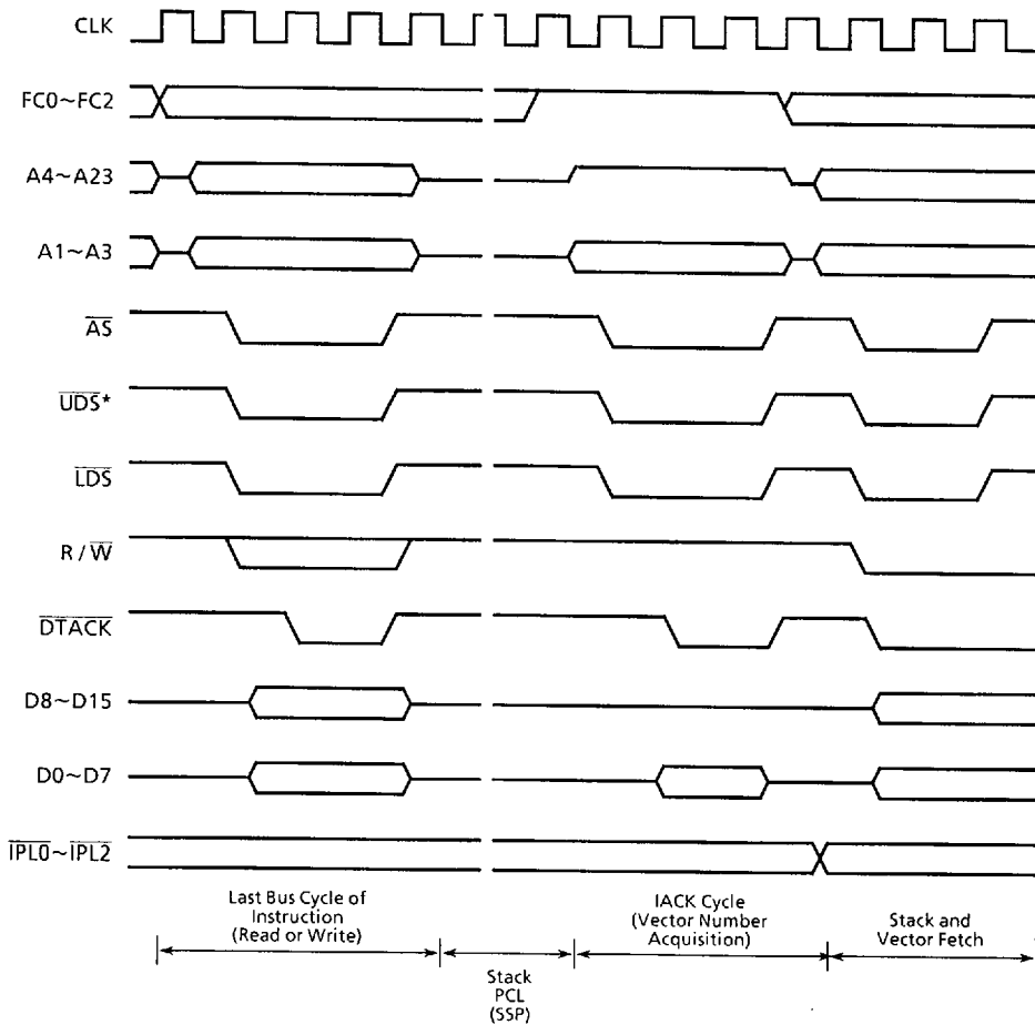
Figure5.6 Interrupt Acknowledge Cycle Timing Diagram
