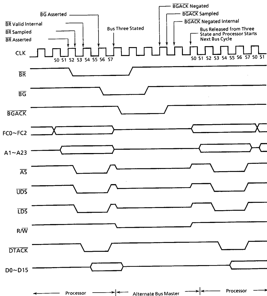
Figure 4.15 Bus Arbitration Timing Diagram – Processor Active
