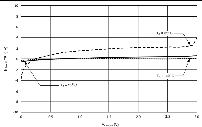
Figure 18. Charge Pump Leakage IF PLL
