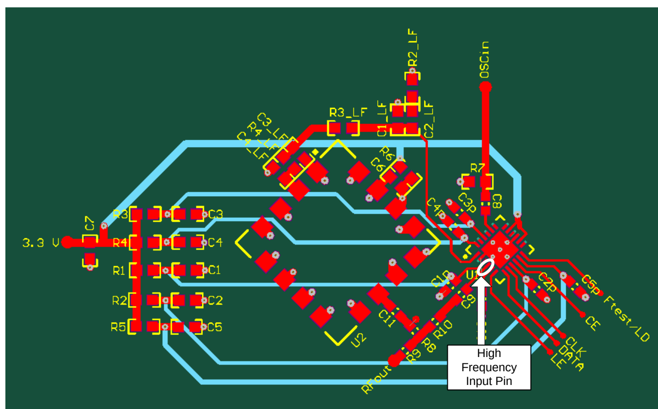
Figure 27. Layout Example
