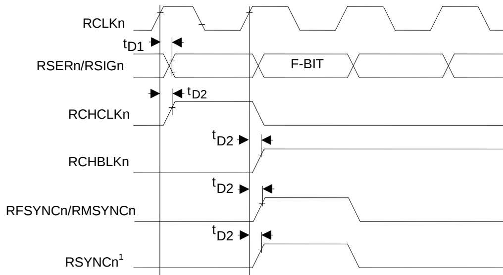
Figure 13-6. Receive Framing Timing—Backplane (T1 Mode)
