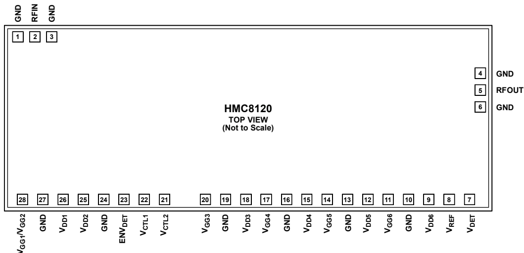
Figure 2. Pad Configuration
