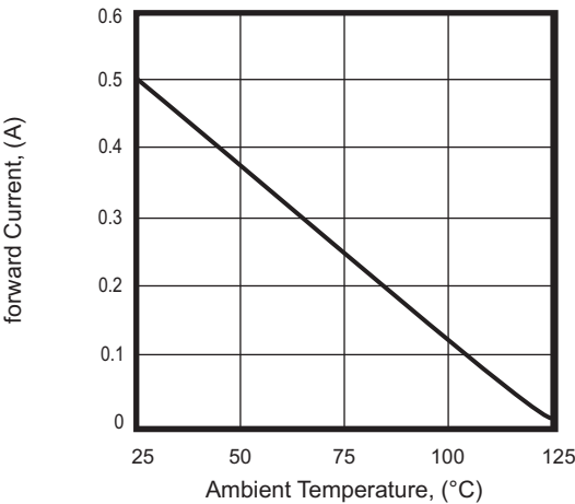
Fig.4 - Power Derating
