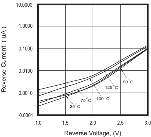
Fig.2 - Reverse Characteristic
