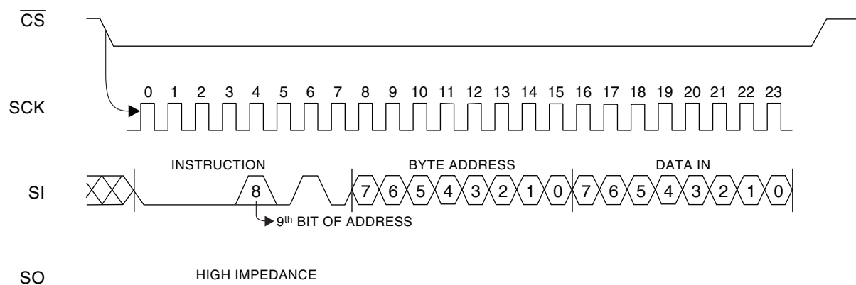
Figure 4-7. WRITE Timing
