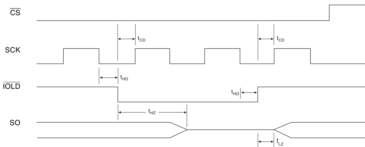
Figure 4-8. \overline{\text{HOLD}} Timing
