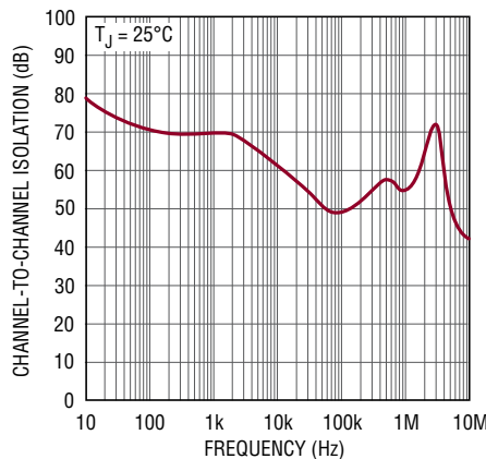
Channel-to-Channel Isolation
