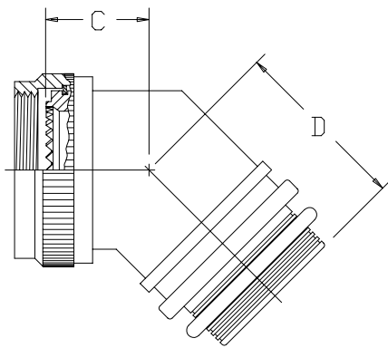
45° ADAPTER-TYPE I
