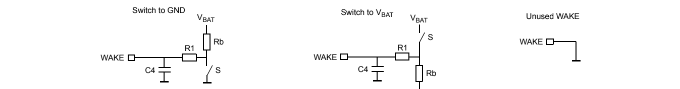
Figure 18. Typical Application and Bus Termination Options and WAKE Pin Configuration
