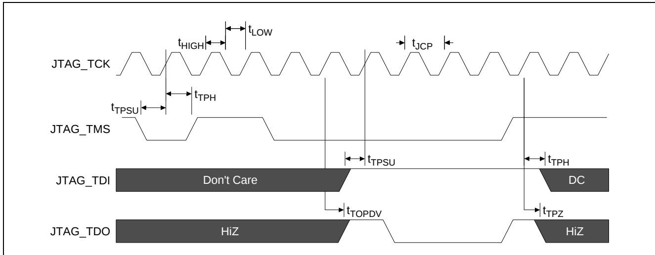
Figure 30 - JTAG Signal Timing
