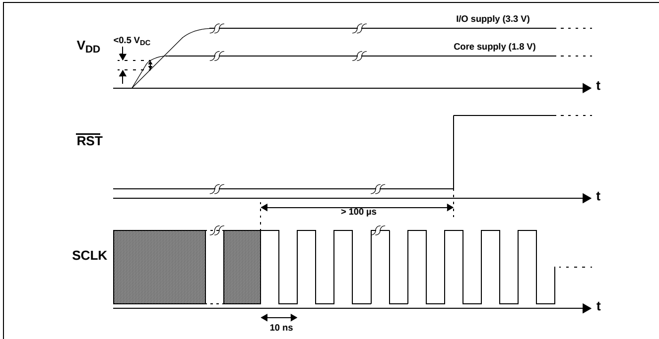
Figure 16 - Powering Up the ZL30301
