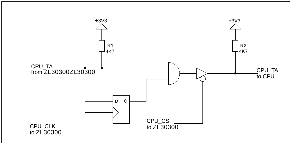
Figure 32 - CPU_TA Board Circuit
