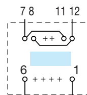
1 Secondary winding 7 8 11 12
