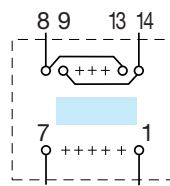
1 Secondary winding 8 9 13 14
