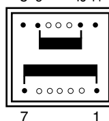
Primary winding
