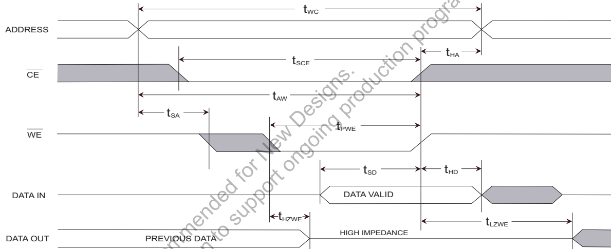
Figure 10. SRAM Write Cycle 2: \overline{CE} Controlled [12, 13]
