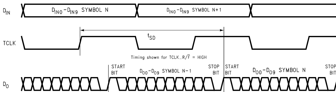
Figure 8. Serializer Delay
