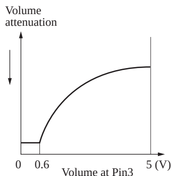
Fig. Volume characteristic of AN5274
