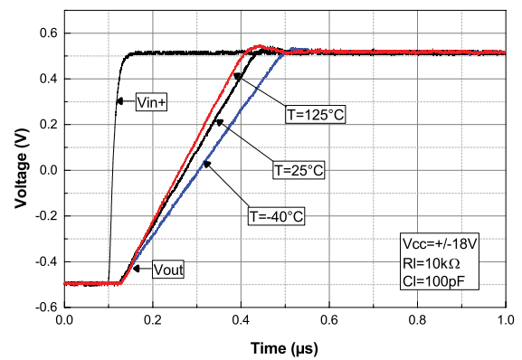
Figure 20. Positive slew rate at V_{CC} = 36\text{ V}
