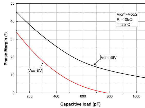
Figure 26. Phase margin vs. capacitive load
