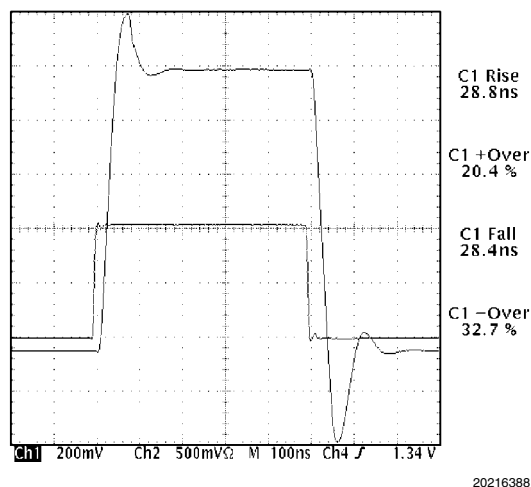
FIGURE 14. R_C = 330\Omega and C = 10 nF, Gain = +1
